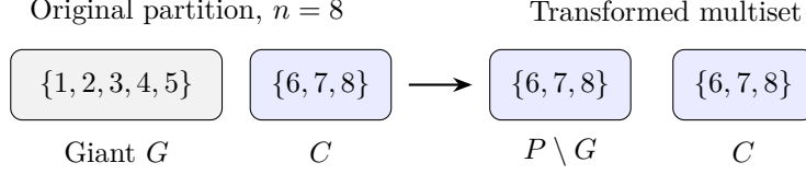
Figure 1: Replacing a giant cell by its complement can duplicate an existing cell. Both occurrences are retained in every overlap sum.
