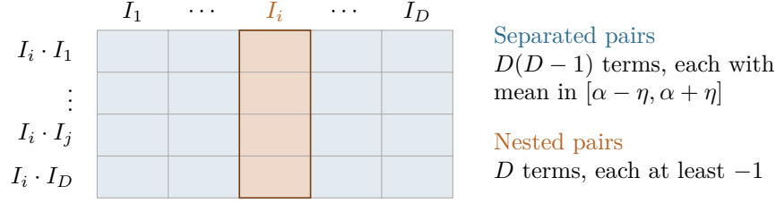
Figure 1: For fixed i , the (j, k) entry is \langle X_{I_i \cdot I_j}, X_{I_k} \rangle . Rows index the children of I_i and columns index all parents; the grid is schematic. Only column i contains nested pairs, a fraction 1/D of the D^2 terms.
