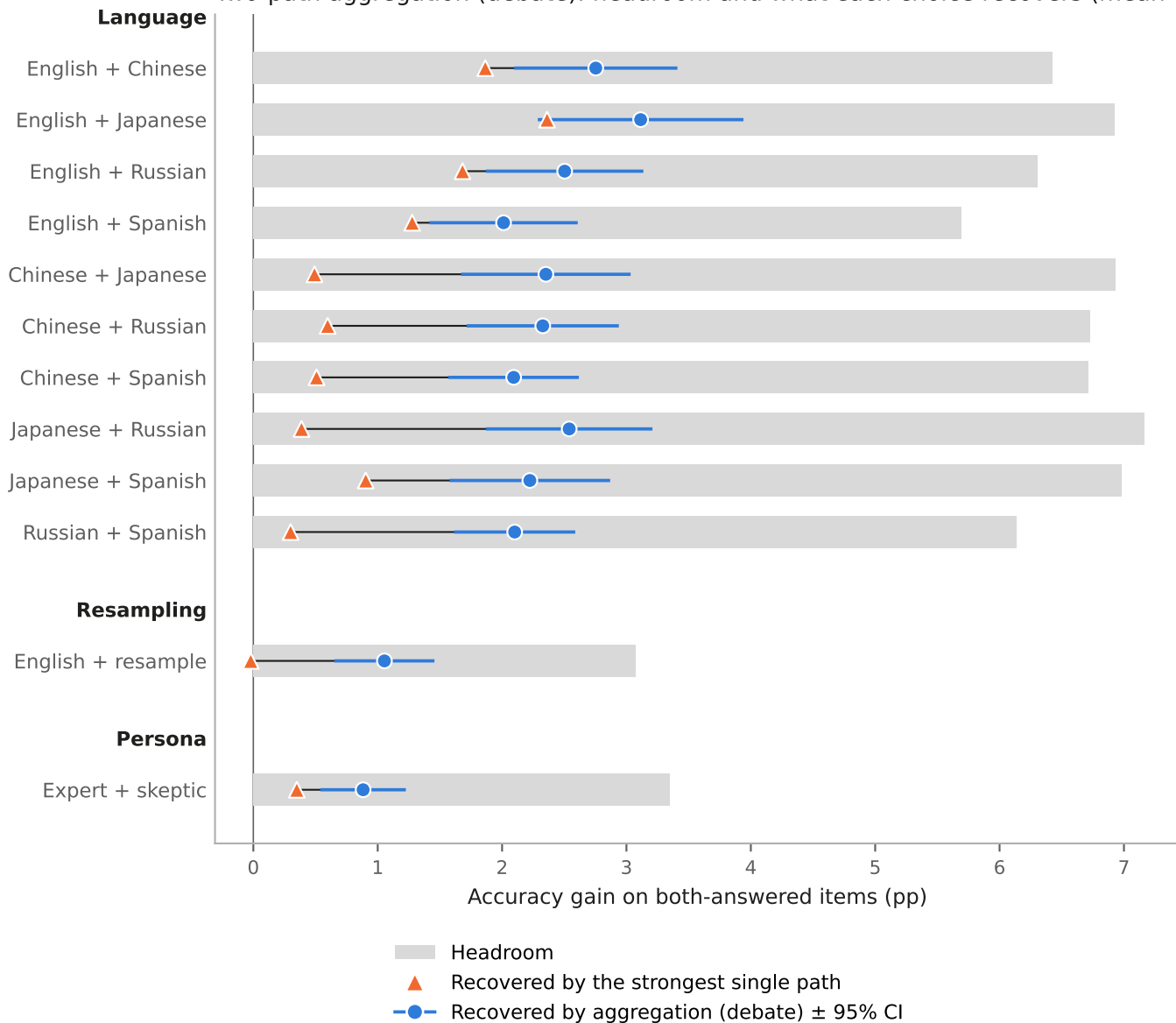
Two-path aggregation (debate): headroom and what each choice recovers (mean of 16 blocks)
