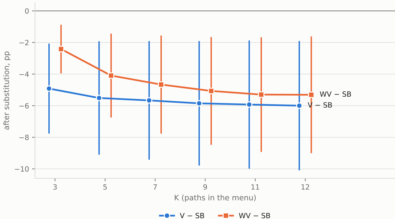
RQ3-GK (b): vote minus strongest single path after substitution, rule A (8 weak blocks)
