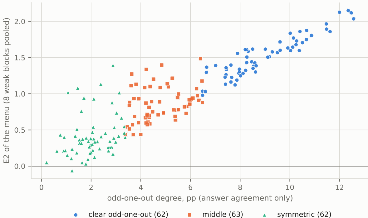
RQ3-GS (b): odd-one-out degree vs E2 of each menu 187 confirmation menus, Spearman +0.89
