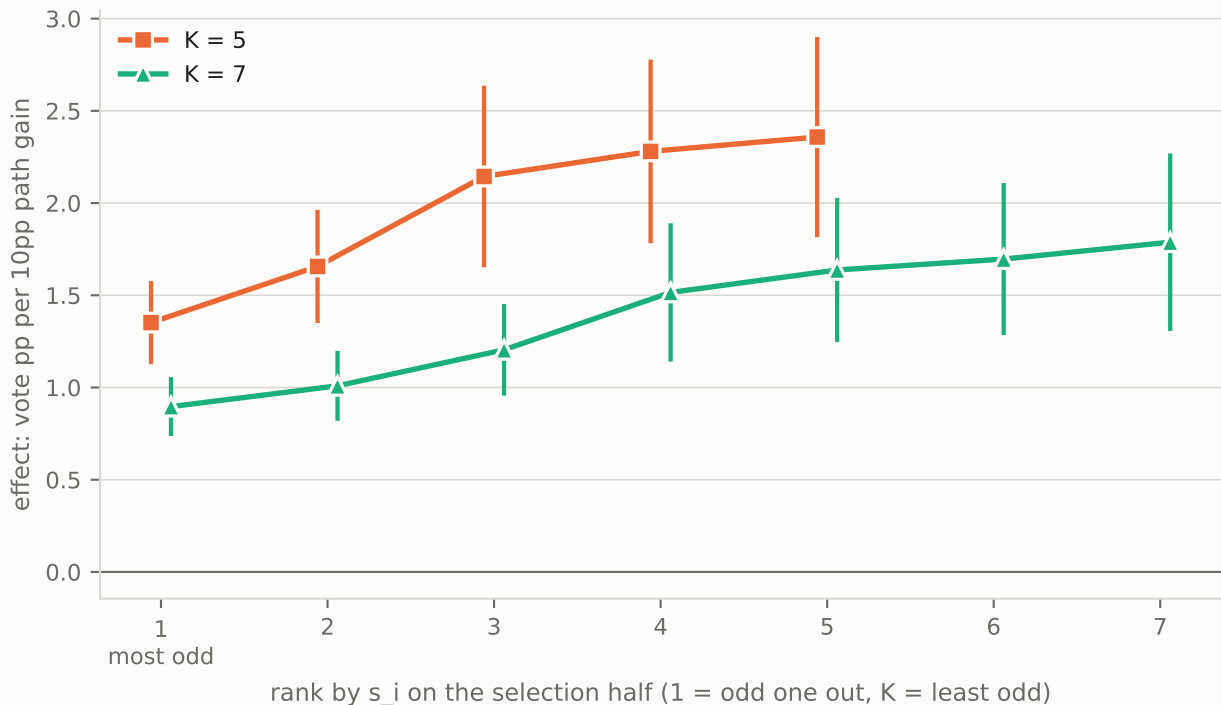
RQ3-GSK (b): effect by odd-one-out rank, rule C 762 confirmation menus per K (8 weak blocks, 95% t interval)
