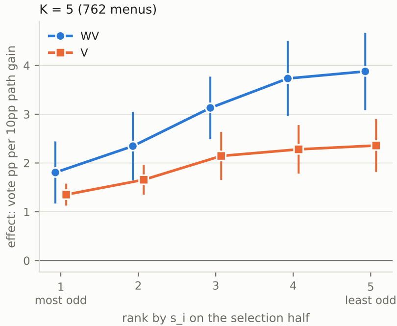
RQ3-GSX (b): effect by odd-one-out rank, rule C (8 weak blocks, 95% t interval)
