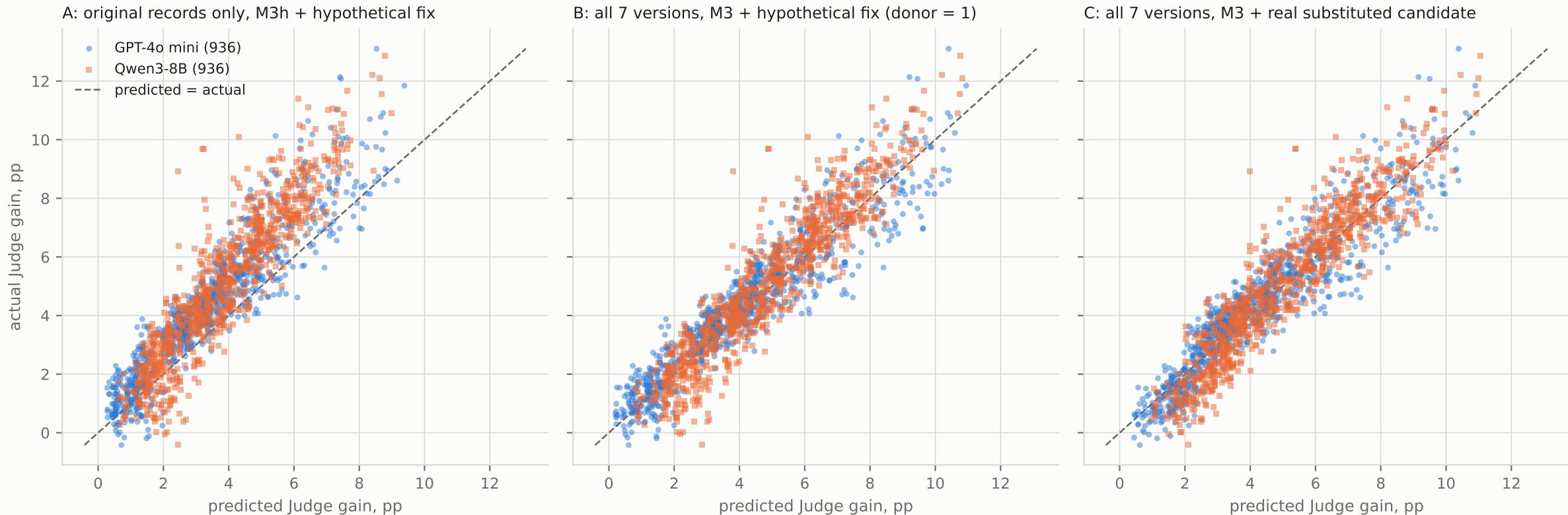
RQ3-GJT (a): predicted vs actual gain per substitution, leave-one-dataset-out (evaluation half, mean of 200 splits)
