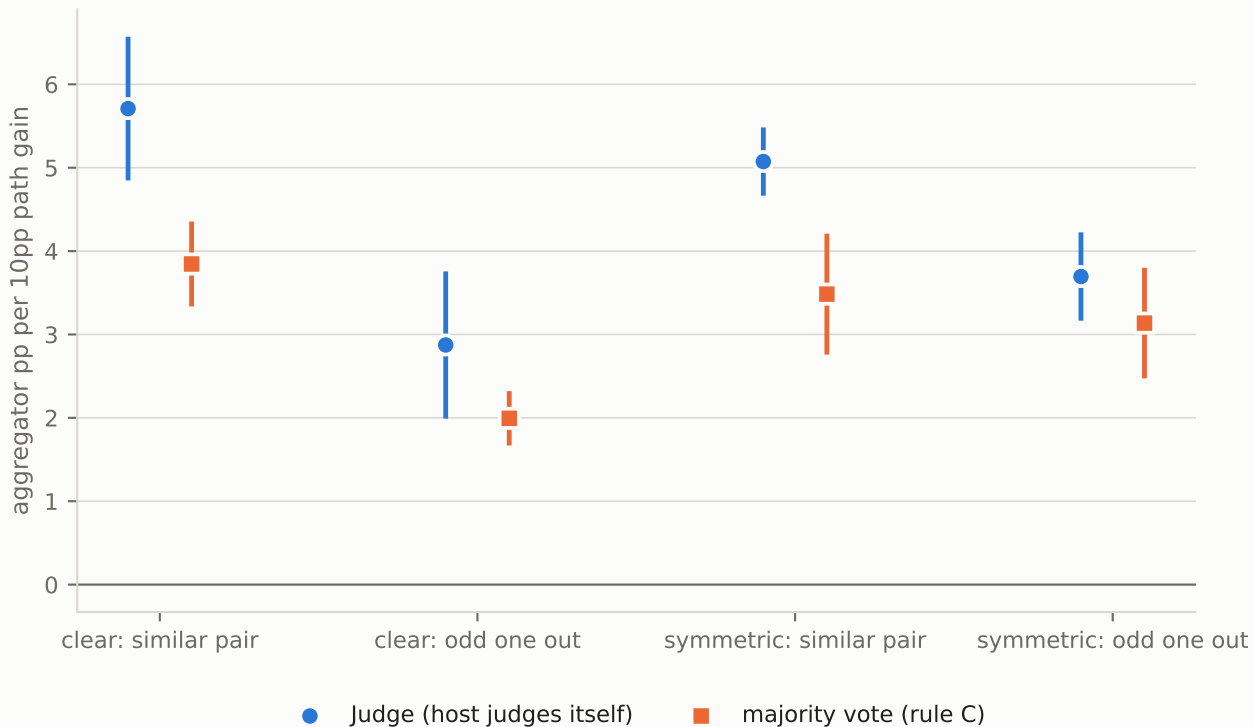
RQ3-GJ (a): effect of improving one path, K = 3 (8 weak blocks, 95% t interval)
