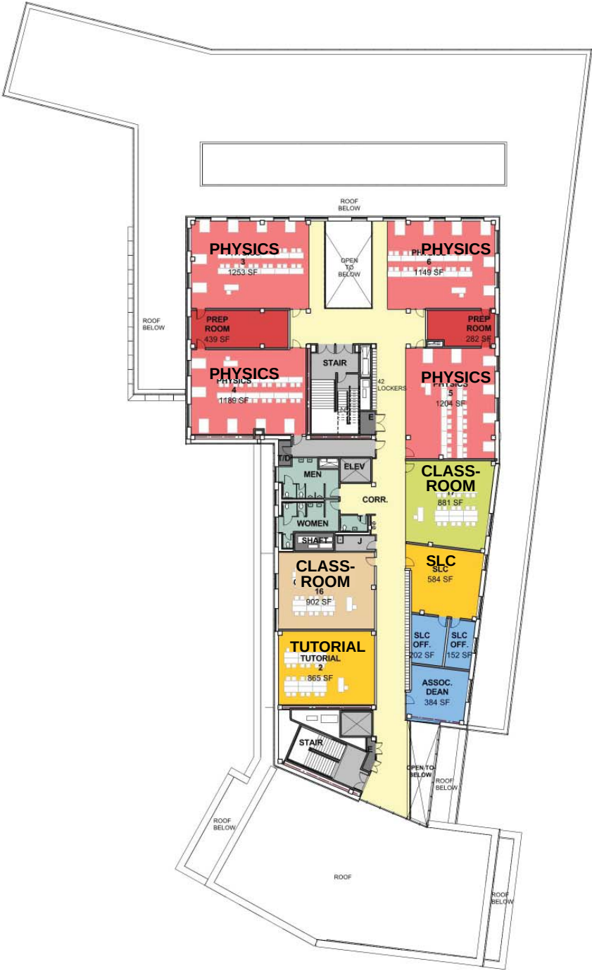
LEVEL 4
