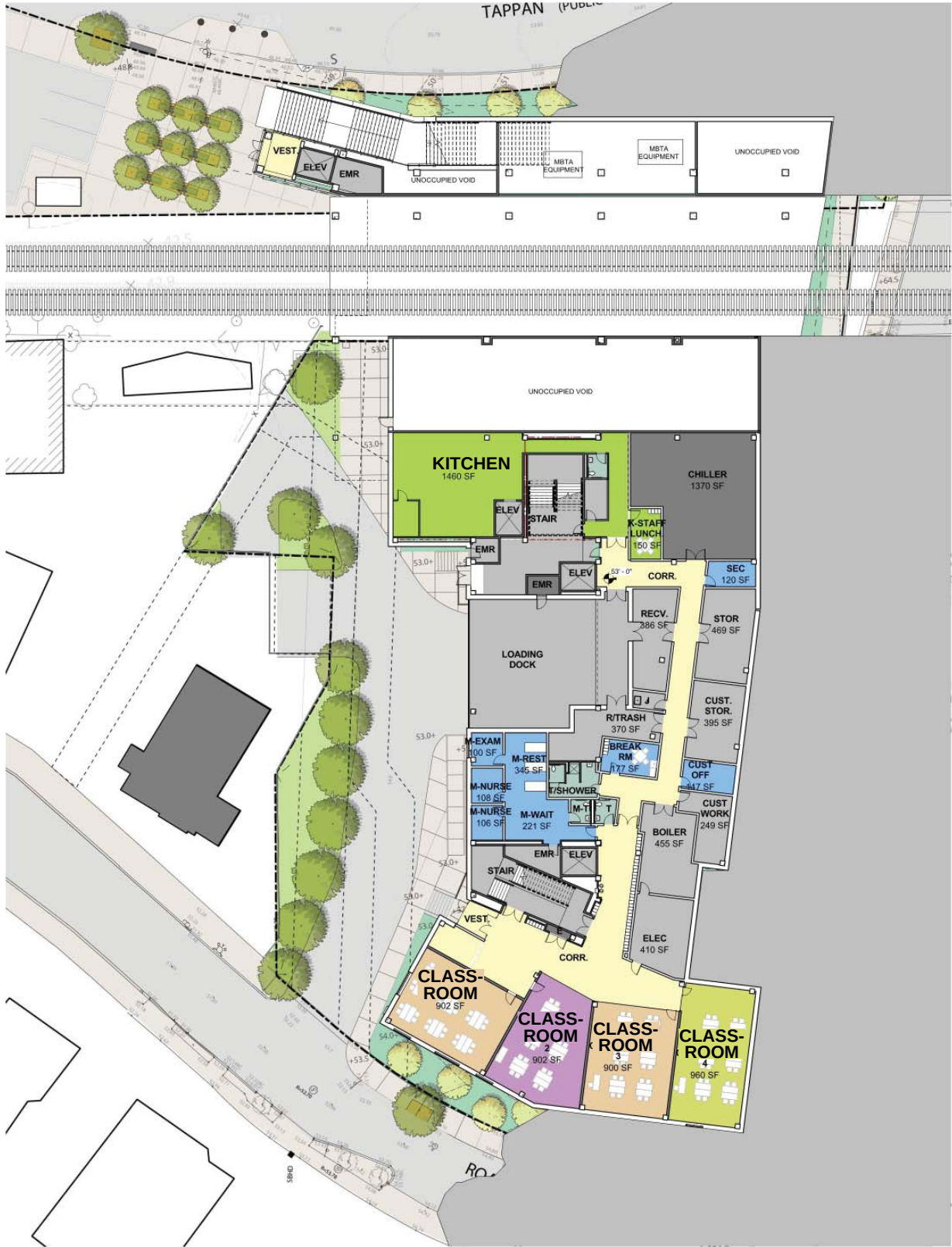
LOWER LEVEL
