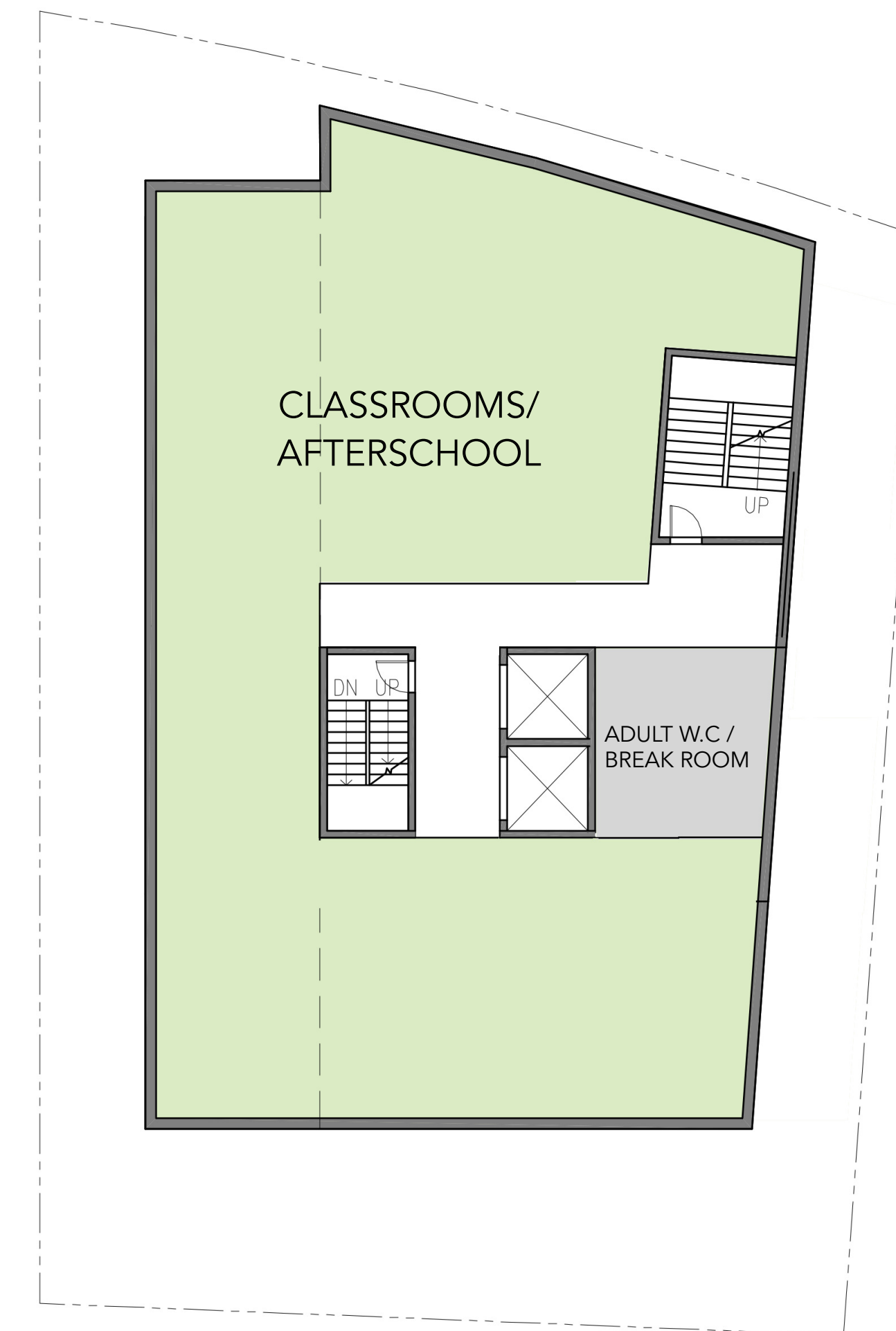
LEVELS 2-4
