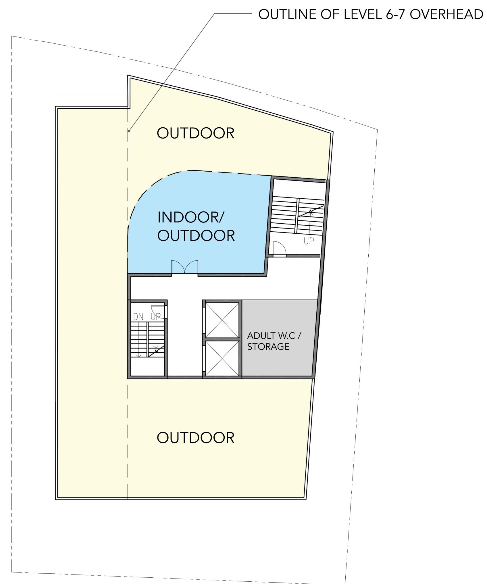
LEVEL 5 - PLAYGROUND
