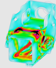
NONLINEAR FEA, TORQUE TUBE CRADLE
