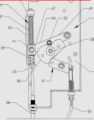
PORTABLE MECH OPERATED CELL
