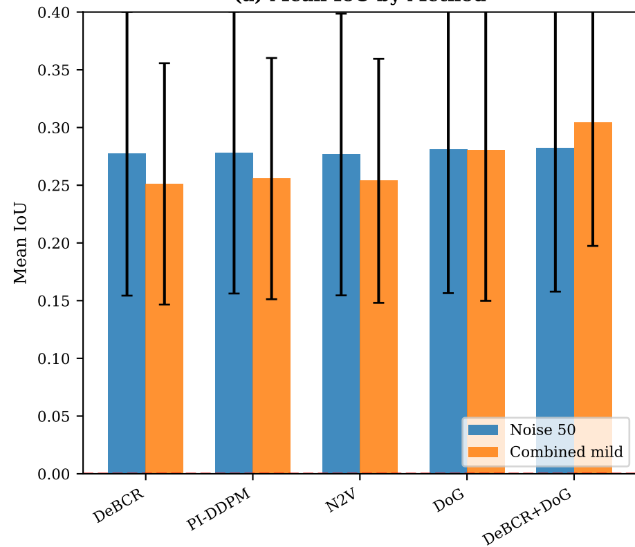
(a) Mean IoU by Method
