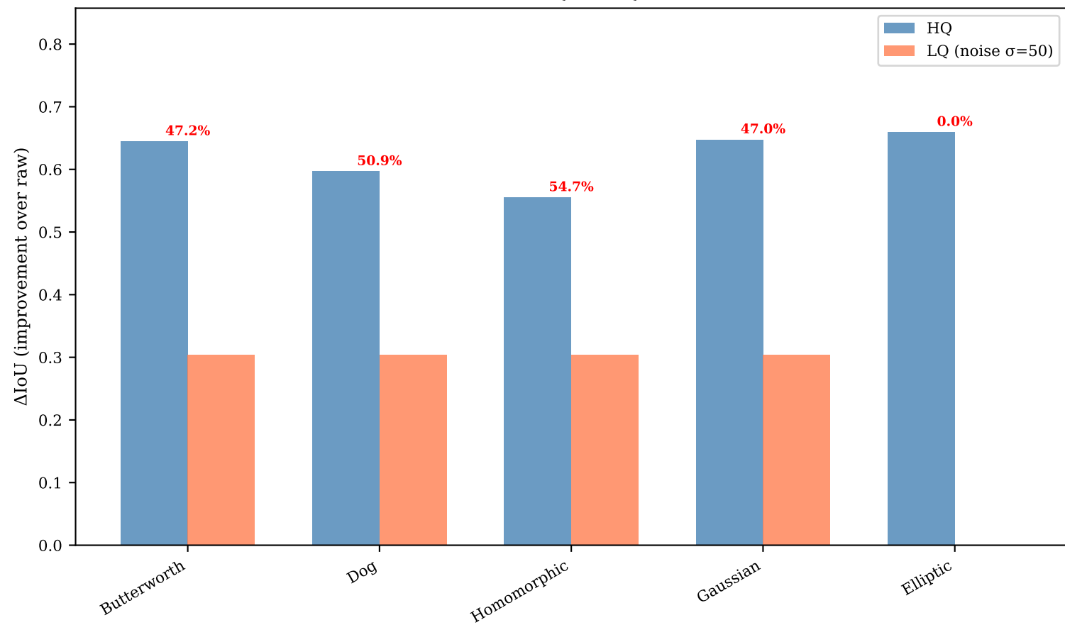
Filter Transfer: HQ vs LQ Performance
