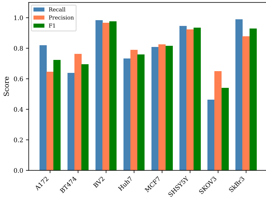
(a) Per-Class Classification Metrics
