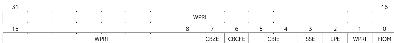
Figure 57. Supervisor environment configuration register ( senvcfg ) for RV32.
