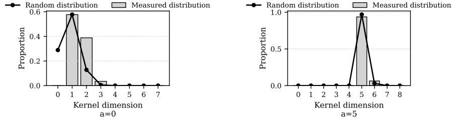
Fig. 1: Empirical distribution of \dim \ker DP_{\text{HFE-IP}}^-(x, \cdot) for n = 32 , d = 2 , r = 1 , N_{\text{samples}} = 10^4 , compared with the theoretical distribution of a random (n-a) \times n binary matrix.
