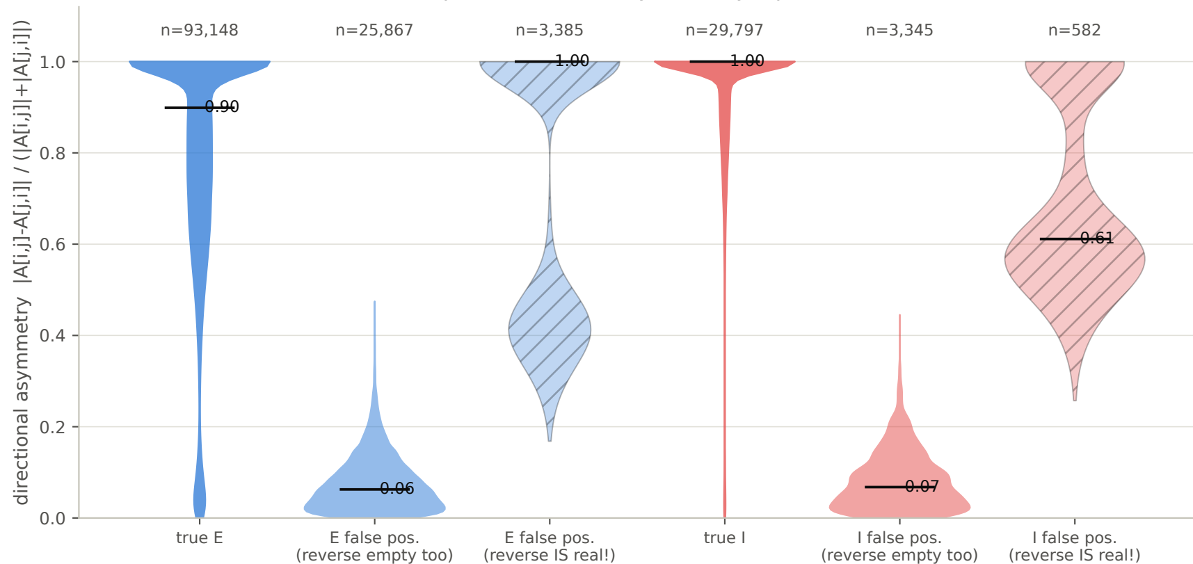
False positives split by reverse-direction truth, N=1250 (single-lag OLS) hatched = this "false positive" is actually a real synapse in the OTHER direction
