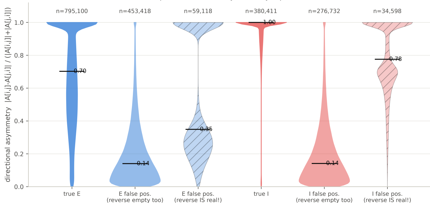
False positives split by reverse-direction truth, N=12500 (single-lag OLS) hatched = this "false positive" is actually a real synapse in the OTHER direction
