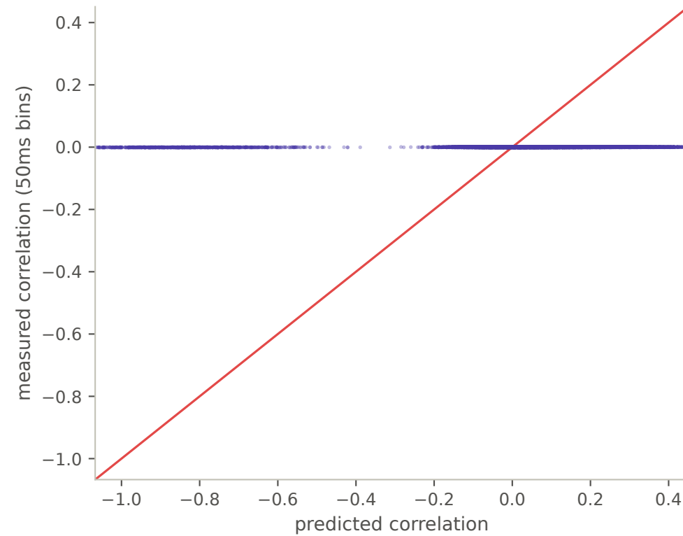
D: correlation, predicted vs simulated ( r=0.40 )
