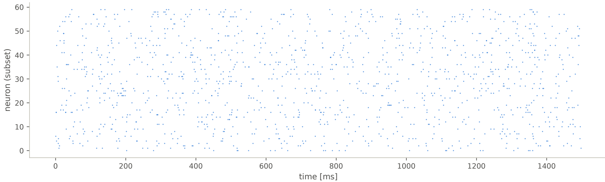
A: raster, 60 neurons (mean rate 14.2 Hz)
