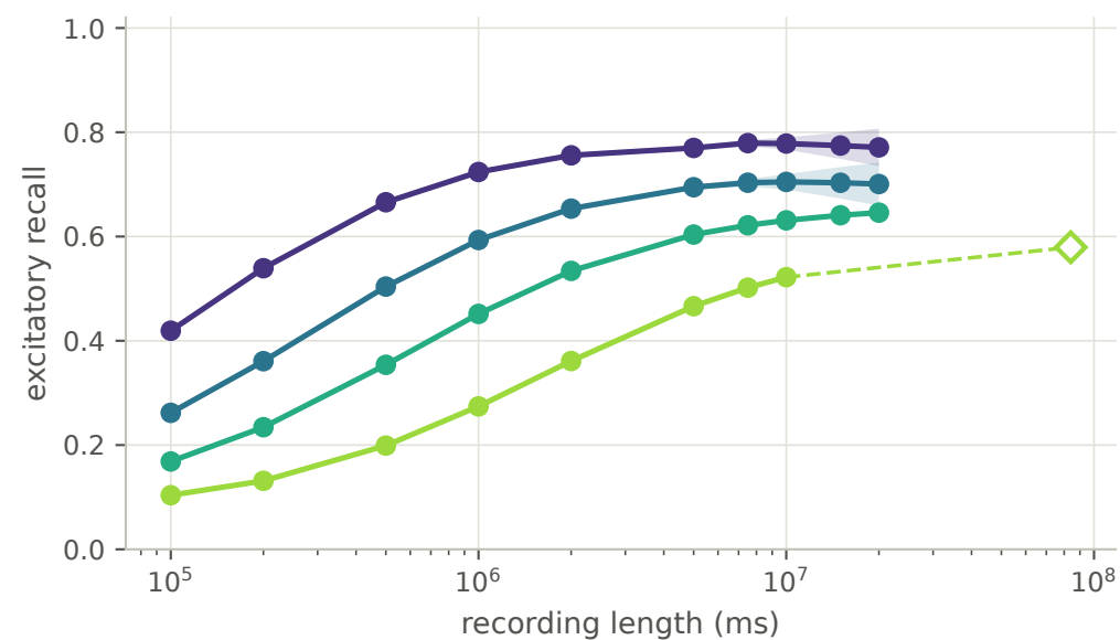
Scaling: recovery is set by data per neuron (matched AI regime, ~14 Hz, OLS)
