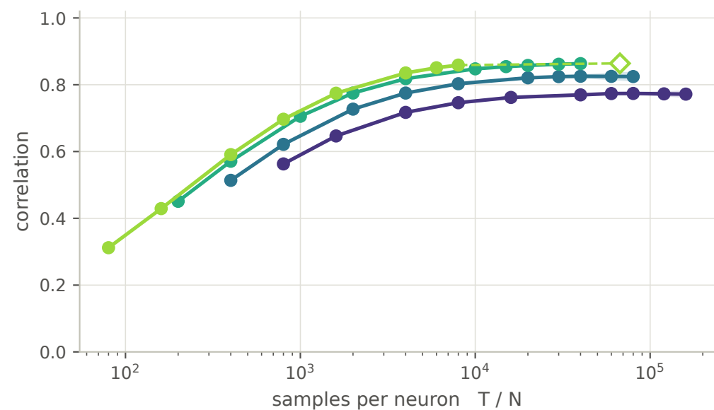
Same measures at matched samples-per-neuron ( T/N ) — does the size gap survive?
