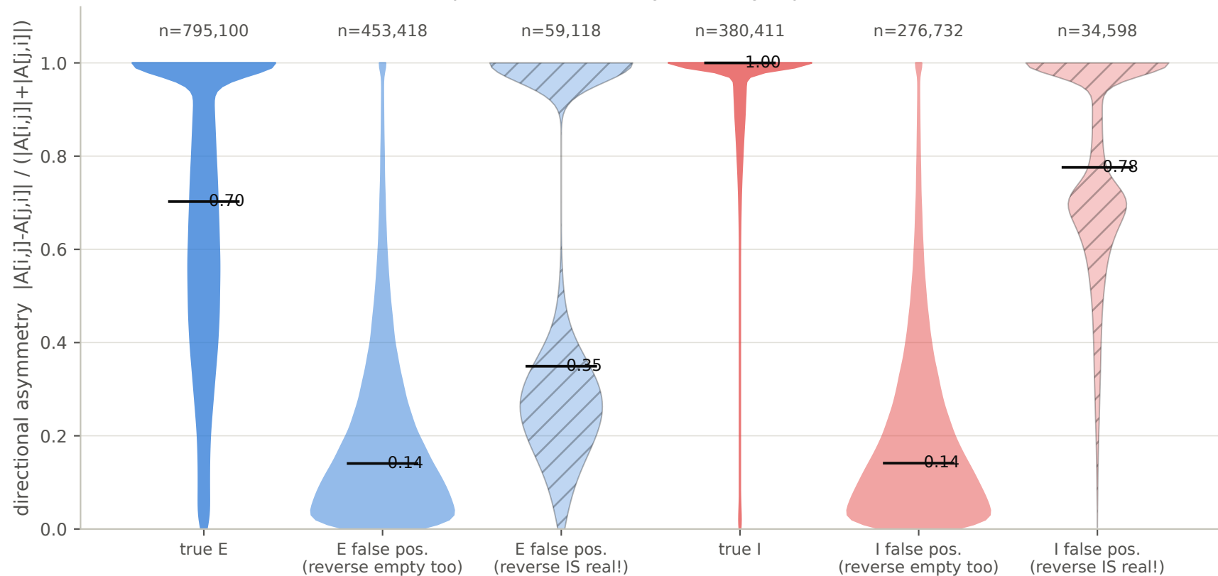
False positives split by reverse-direction truth, N=12500 (OLS) hatched = this "false positive" is actually a real synapse in the OTHER direction
