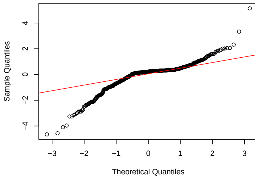
QQ-Plot (Deviance)
