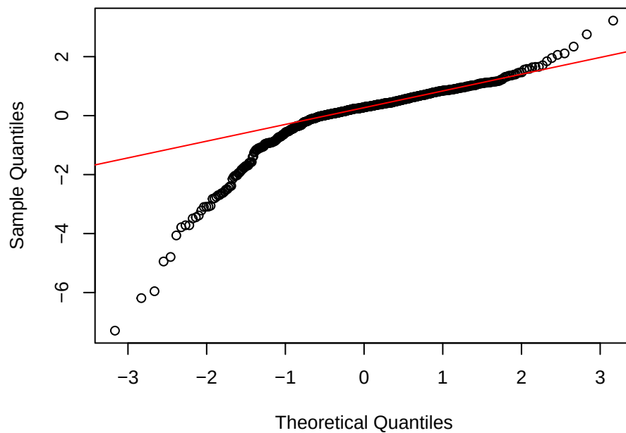
QQ-Plot (Pearson)
