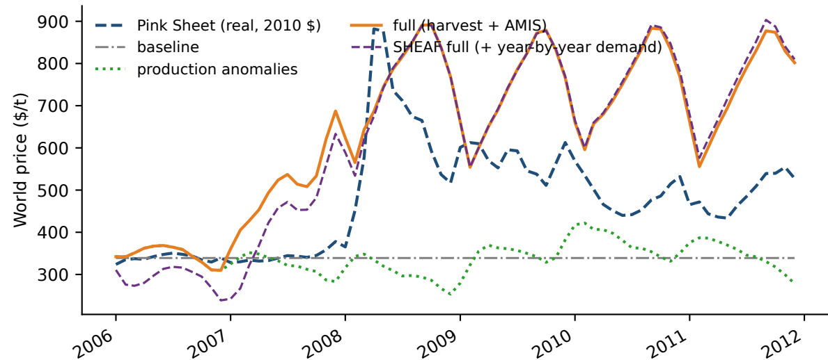
Rice world price — Agrimate scenario split
