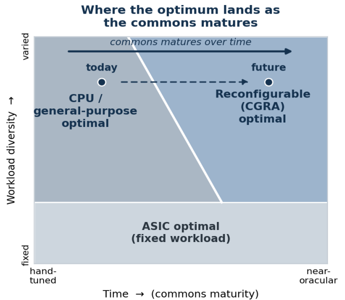
Figure 5. Where the optimum lands. Over the two axes that actually decide the choice — the maturity of the shared optimization commons (which grows over time, accelerated by machine intelligence) and workload diversity — fixed ASICs remain optimal only for stable, high-volume workloads; the large high-diversity space currently defaults to general-purpose silicon because the commons is weak; and as the commons matures the reconfigurable-optimal region sweeps left into that territory. The boundary is conceptual — pinning down its real position is exactly what the whole-system characterization of §12 would enable.
