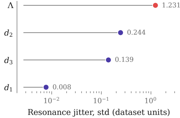
Fig. S2 Resonance jitter attributable to each geometric variable at 3% tolerance, on a logarithmic scale. The lattice pitch (highlighted) dominates by more than a factor of five over the next variable and by two orders of magnitude over the innermost holes.
