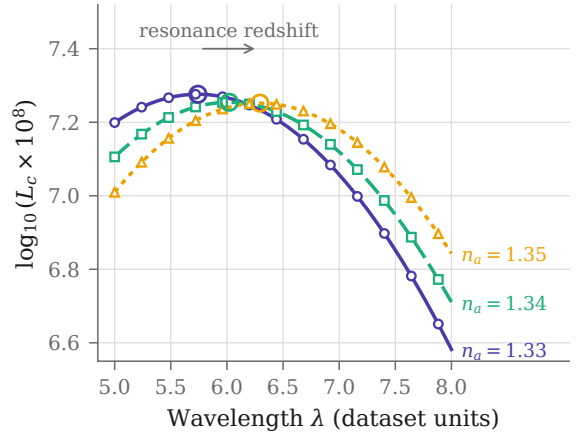
Fig. 4 Predicted confinement-loss spectra at fixed geometry for the three analyte indices. Rings mark the predicted resonance. The peak moves monotonically to longer wavelengths as n_a increases, in uniform steps of 0.276 dataset units per 0.01 refractive index unit.
