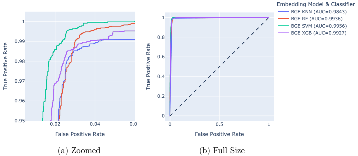
Figure B.1: BGE ROC Curves for Finalist Classifiers with Test Data
