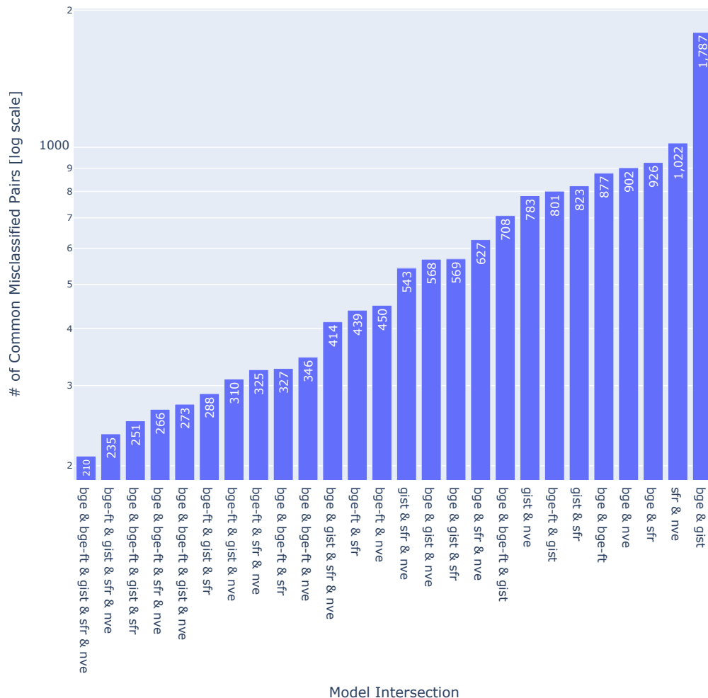
Figure 4.9: Number of common misclassified pairs between all model combinations on the test dataset. The high counts of common errors across different models point to similar challenges inherent in the data.
