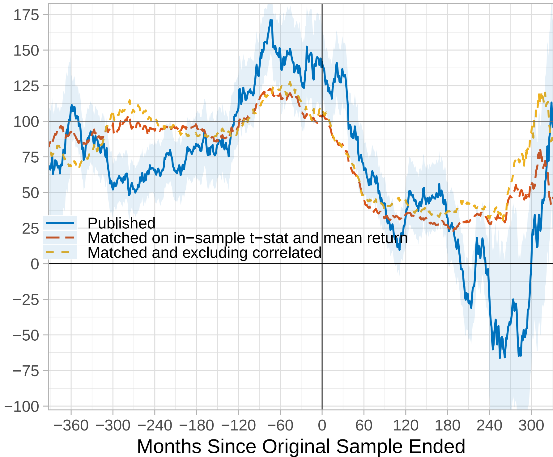
Trailing 5-Year Mean Return (bps p.m.)
