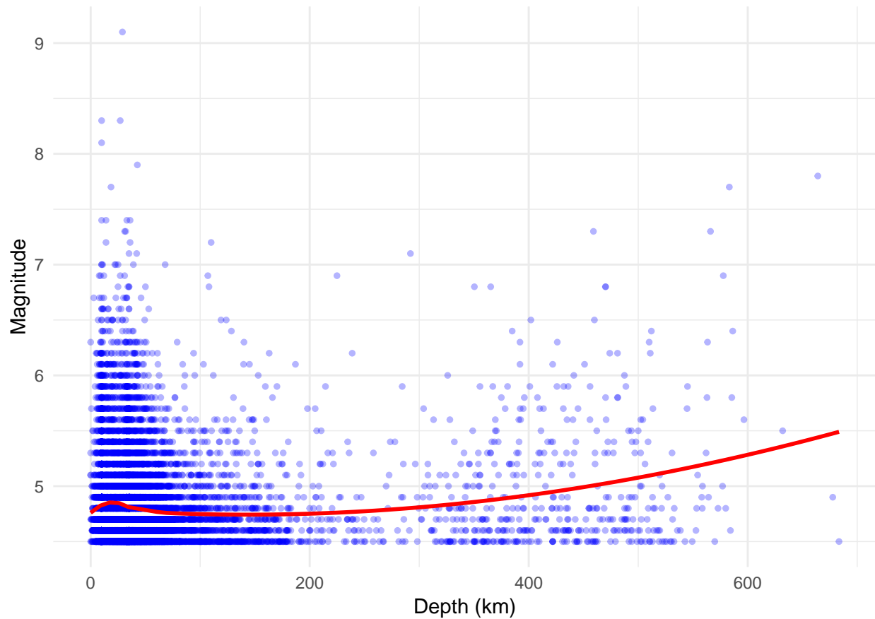
Earthquake depth vs magnitude (Japan, 2001–2018)
