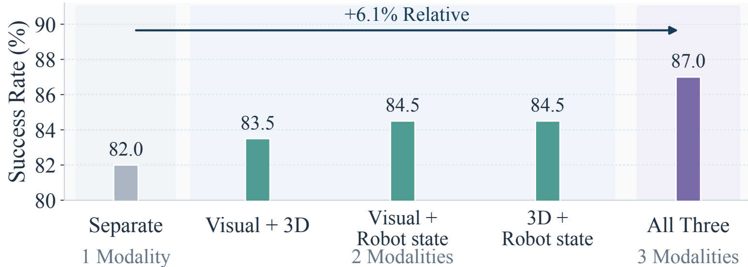
(b) RL Bench
