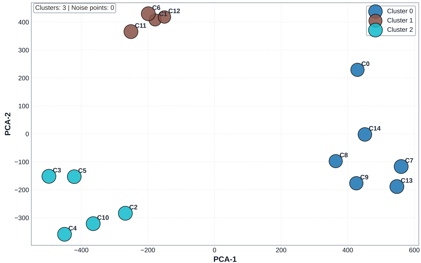
round0weights: HDBSCAN Clusters on PCA Features
