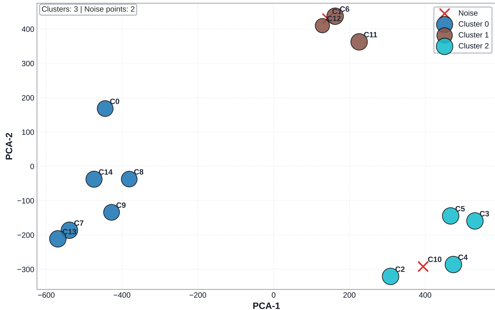
round1weights: HDBSCAN Clusters on PCA Features
