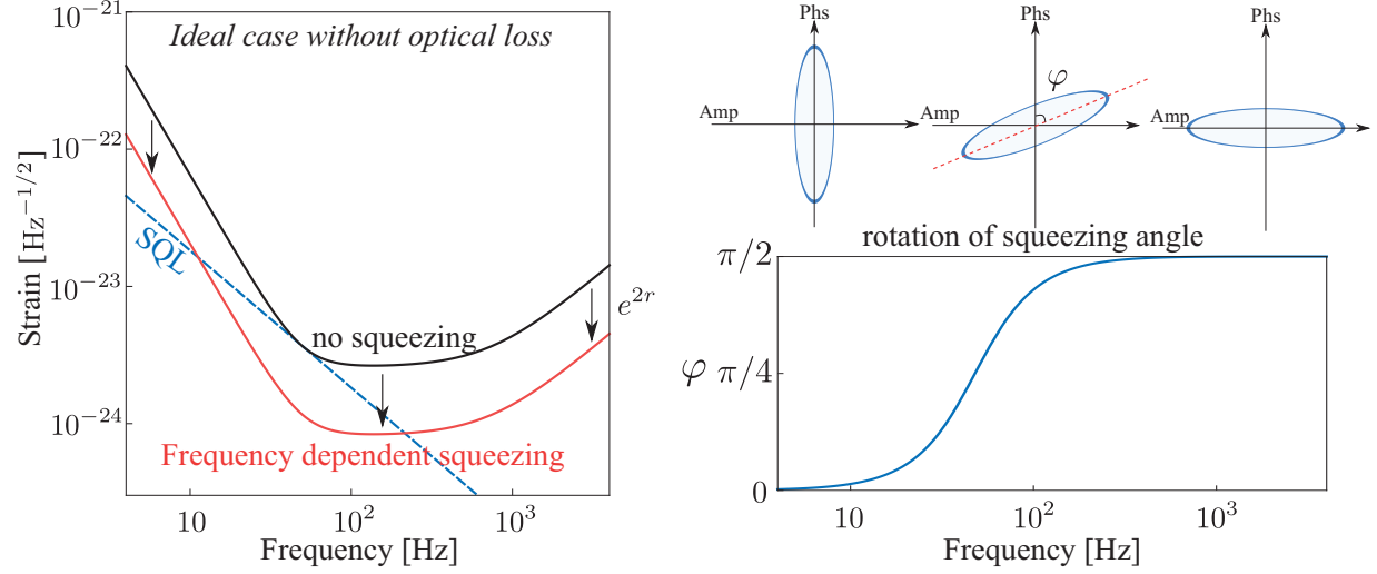
Figure 13: Noise spectrum for frequency-dependent squeezing (left) and rotation of the squeeze angle (right).
