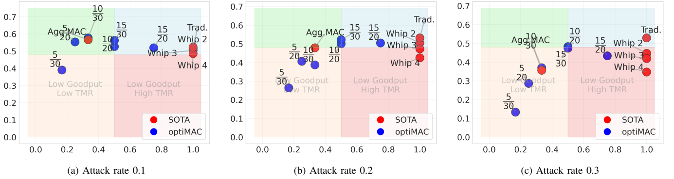
Fig. 12: Goodput (y-axis) vs. TMR (x-axis) of 5G experiments where more than 80% of Traditional MAC's Goodput is considered high. State-of-the-art (SOTA) includes traditional, progressive, and aggregate MAC vs. the optiMAC.
