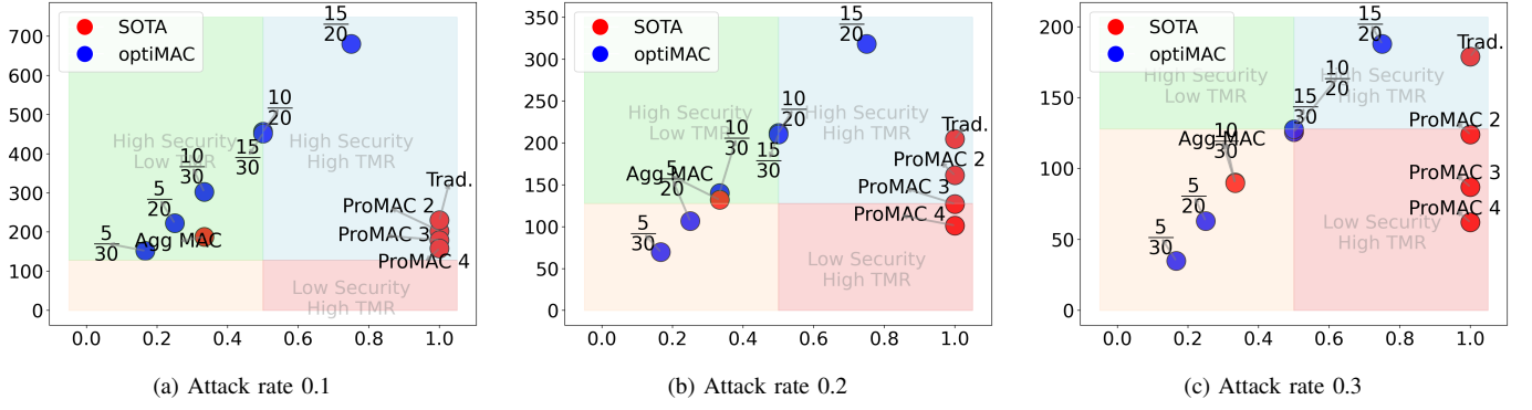
Fig. 9: TbpM (y-axis) vs. TMR (x-axis) of WiFi experiments with 256-bit tags (128 or higher TbpM is high security). State-of-the-art (SOTA) includes traditional, progressive, and aggregate MAC vs. the optimal by optiMAC.
