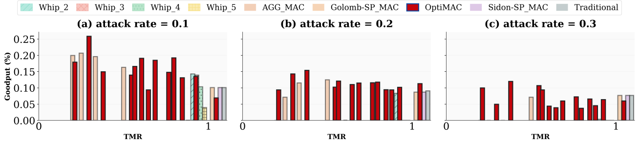
Fig. 7: Periodic jamming simulation for message size of 32 bits and security requirements of 256 bits. OptiMAC is the only scheme that can provide adaptive solutions for TMR between 1/2 and 1.
