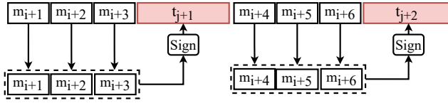
Fig. 3: Aggregate Messages [8]
