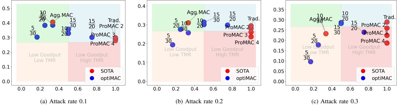
Fig. 10: Goodput (y-axis) vs. TMR (x-axis) of WiFi experiments where more than 80% of Traditional MAC's Goodput is considered high. State-of-the-art (SOTA) includes traditional, progressive, and aggregate MAC vs. the optimal by optiMAC.
