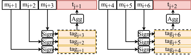
Fig. 2: Aggregate MAC [10]
