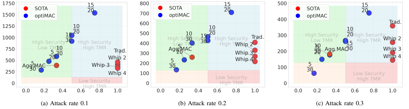
Fig. 8: TbpM (y-axis) vs. TMR (x-axis) of 5G experiments with 512-bit tags (256 or higher TbpM is high security). State-of-the-art (SOTA) includes traditional, progressive, and aggregate MAC vs. the optiMAC.
