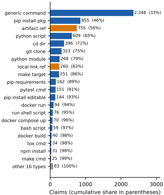
(a) Claim types (N = 7,034)
