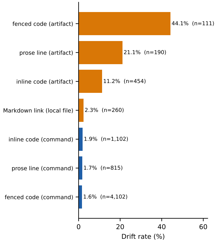
(b) Drift rate by surface context
