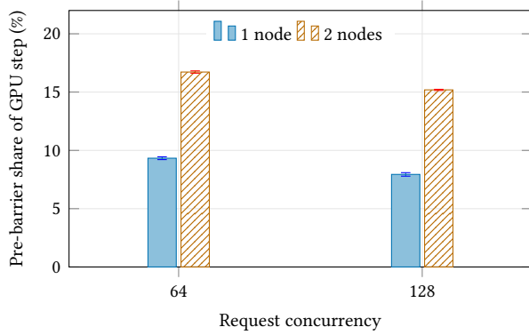
Figure 4. Qwen3-30B-A3B decode at fixed EP8. Pre-barrier intervals for Dispatch and Combine are paired with the same rank’s GPU step. Error bars describe three client windows, not server restarts.
