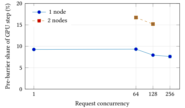
Figure 4. Qwen3-30B-A3B decode at fixed EP8. Each point sums the pre-barriers from 48 Dispatch and 48 Combine calls in one sampled GPU step. The single-node sweep covers concurrency 1–256; cross-node measurements cover 64 and 128. At concurrency 1, one rank is active. Lines connect measured points. Error bars show variation across three client windows.
