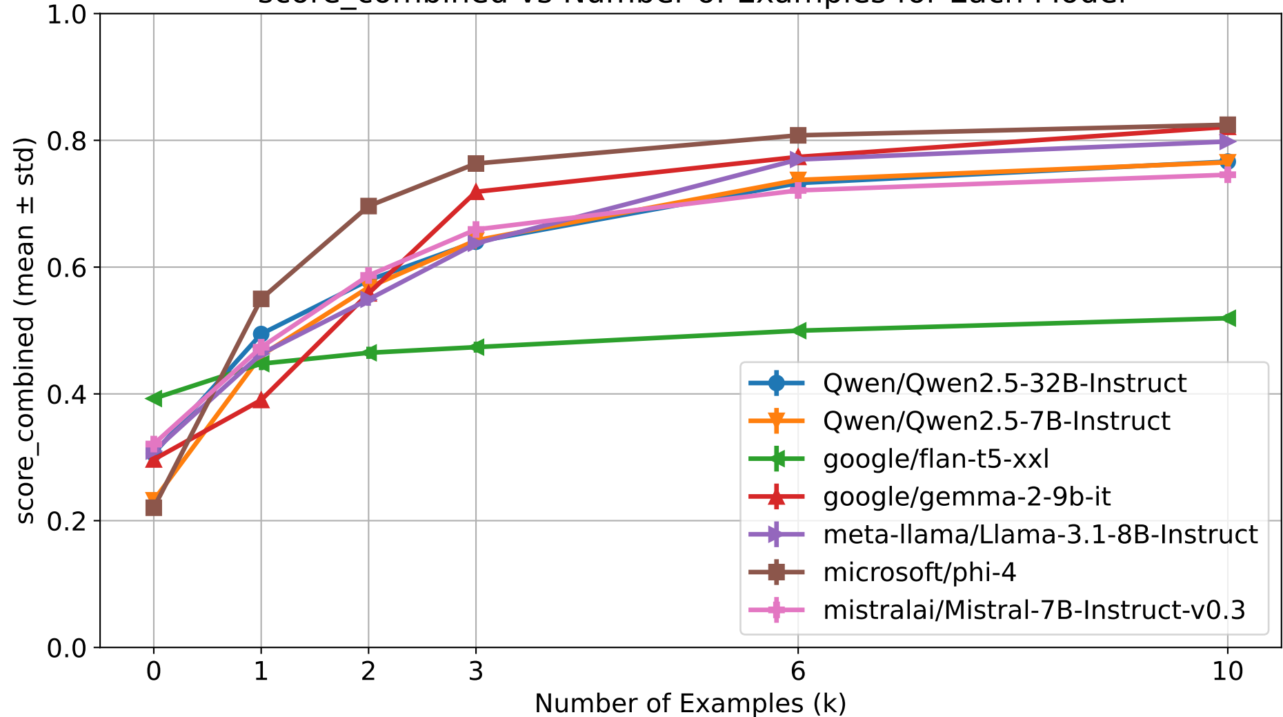
score_combined vs Number of Examples for Each Model
