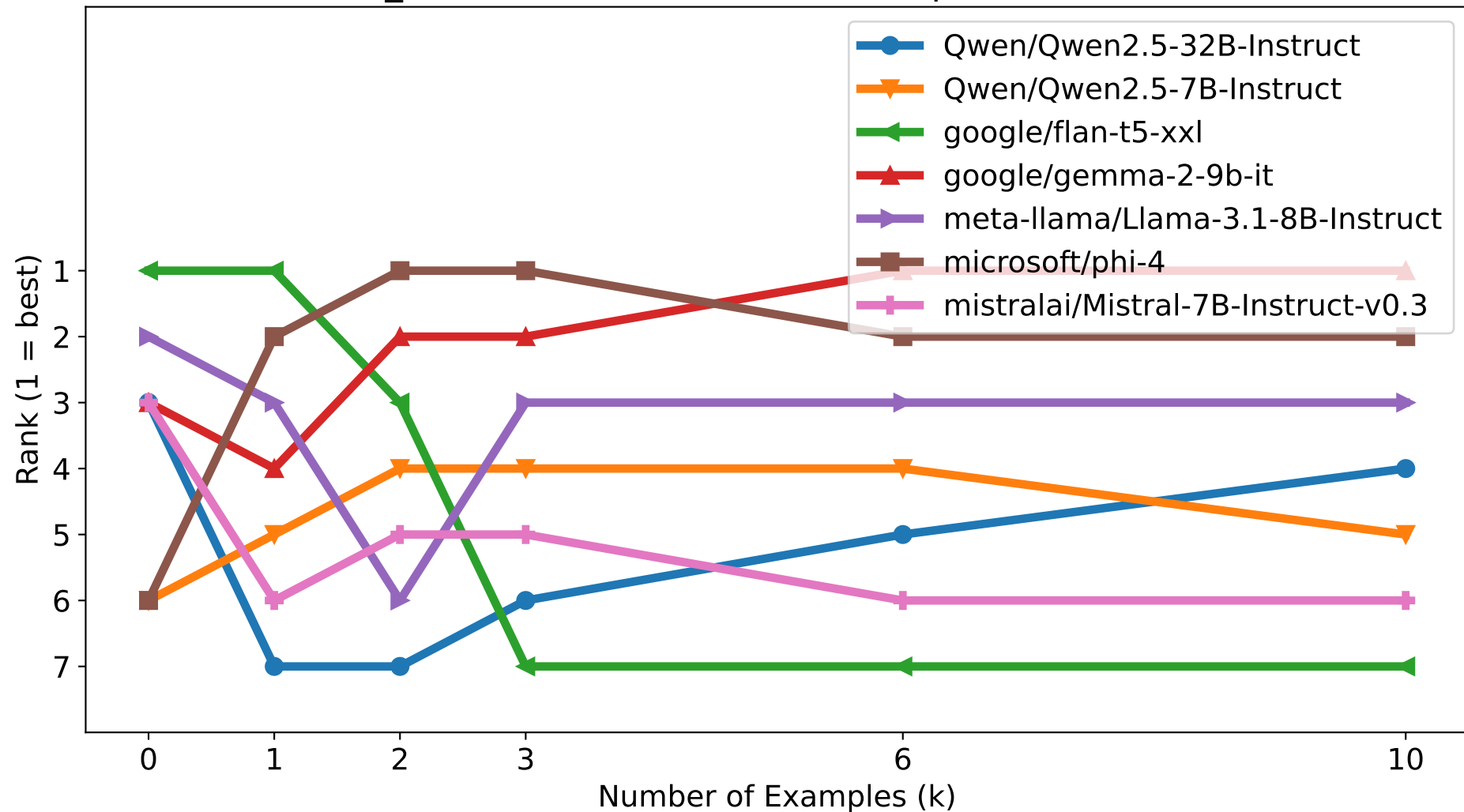
score_em: Rank vs Number of Examples for Each Model
