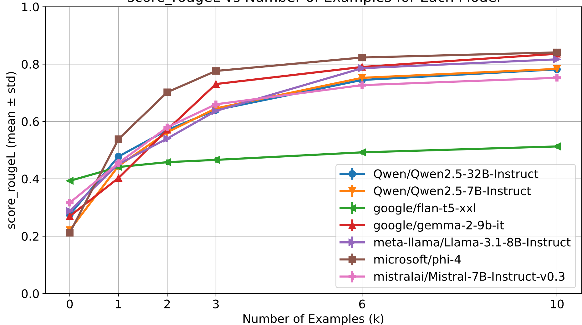
score_rougeL vs Number of Examples for Each Model
