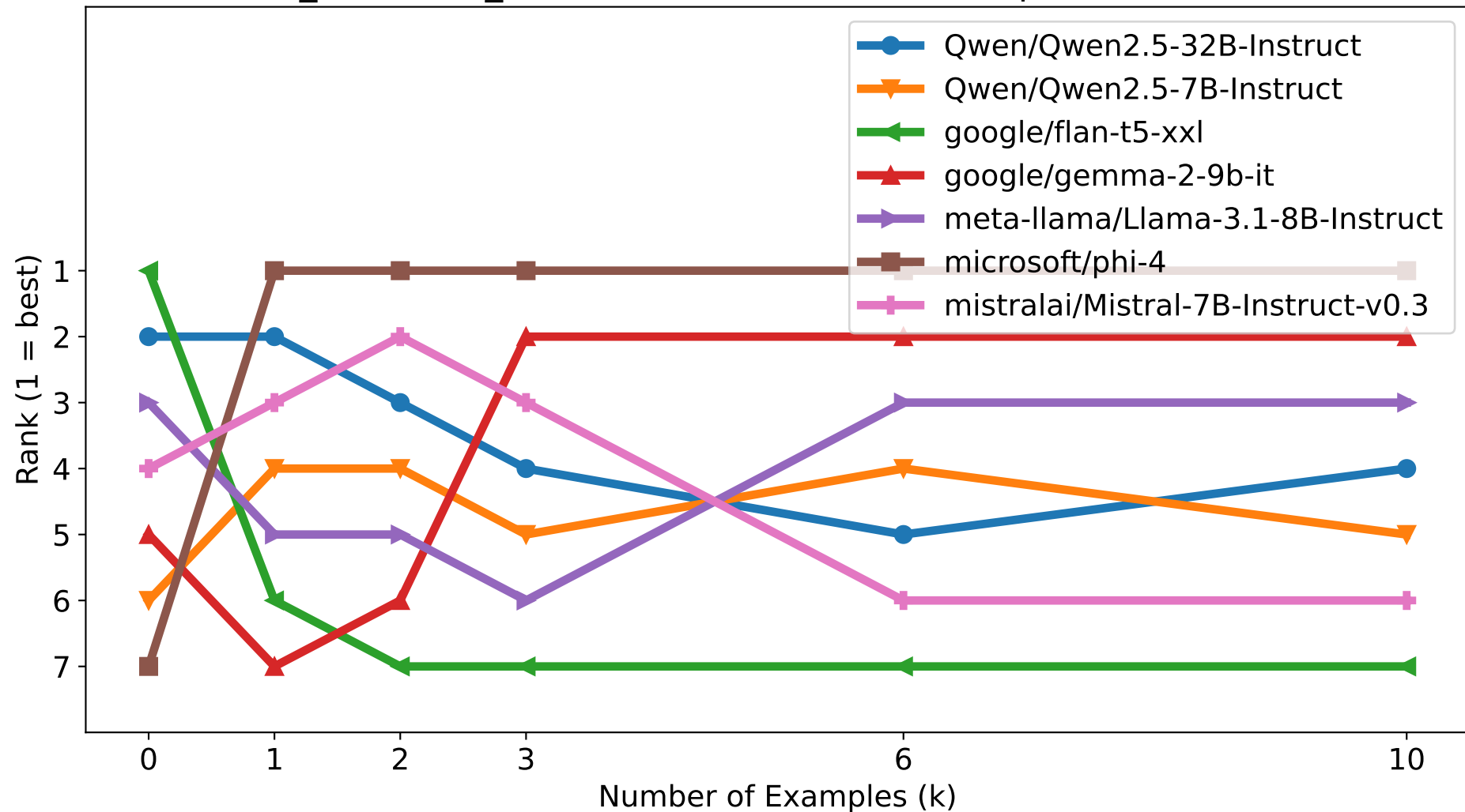
score_bertscore_F1: Rank vs Number of Examples for Each Model
