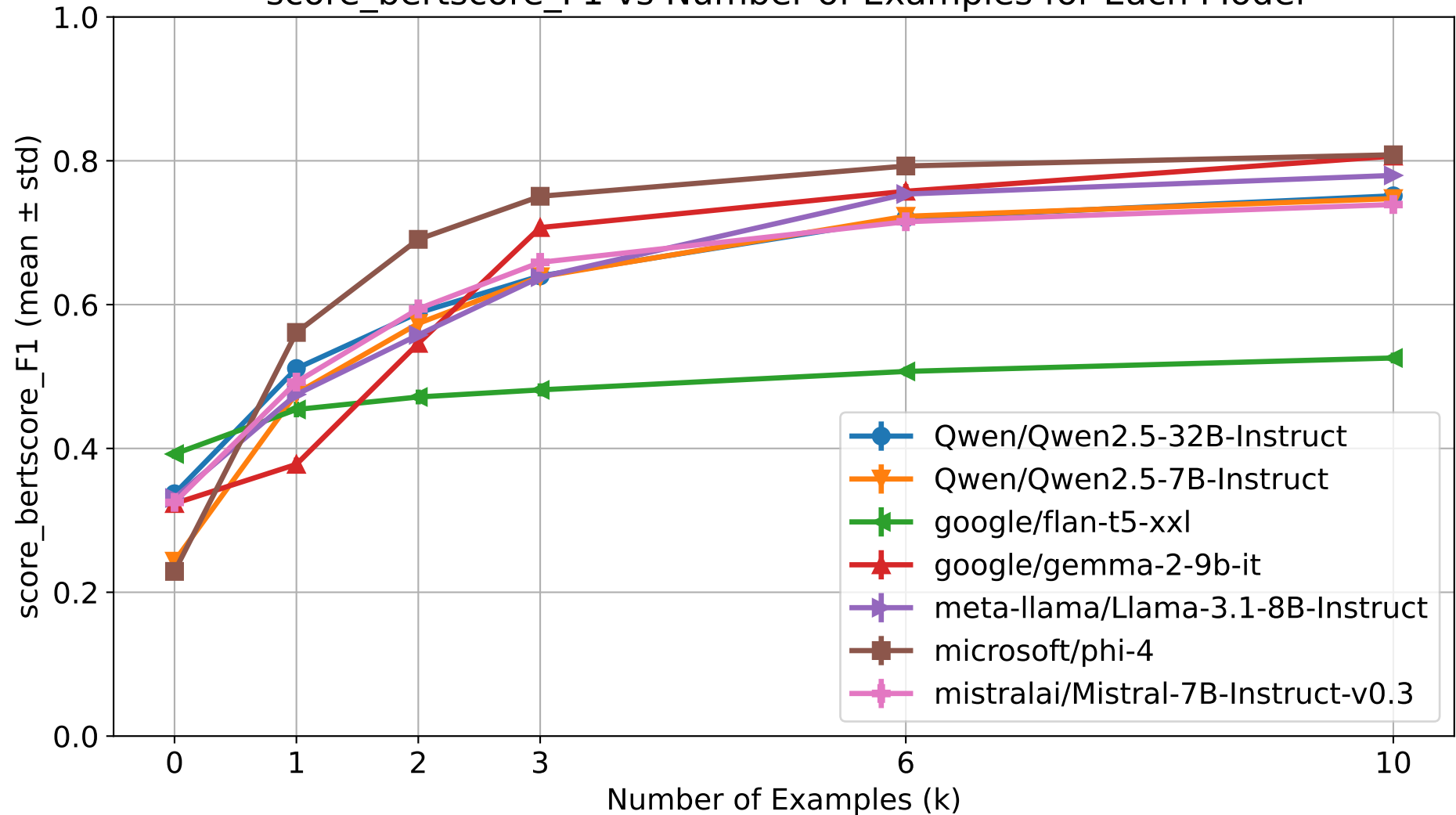
score_bertscore_F1 vs Number of Examples for Each Model
