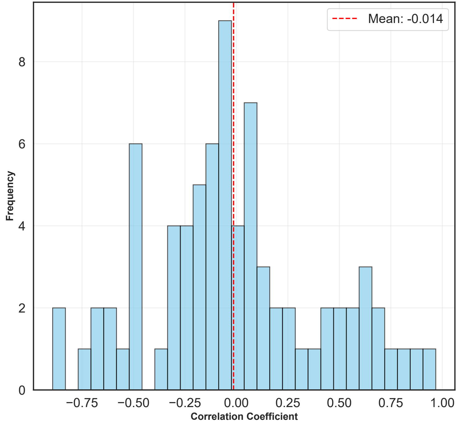
Distribution of Correlation Coefficients
