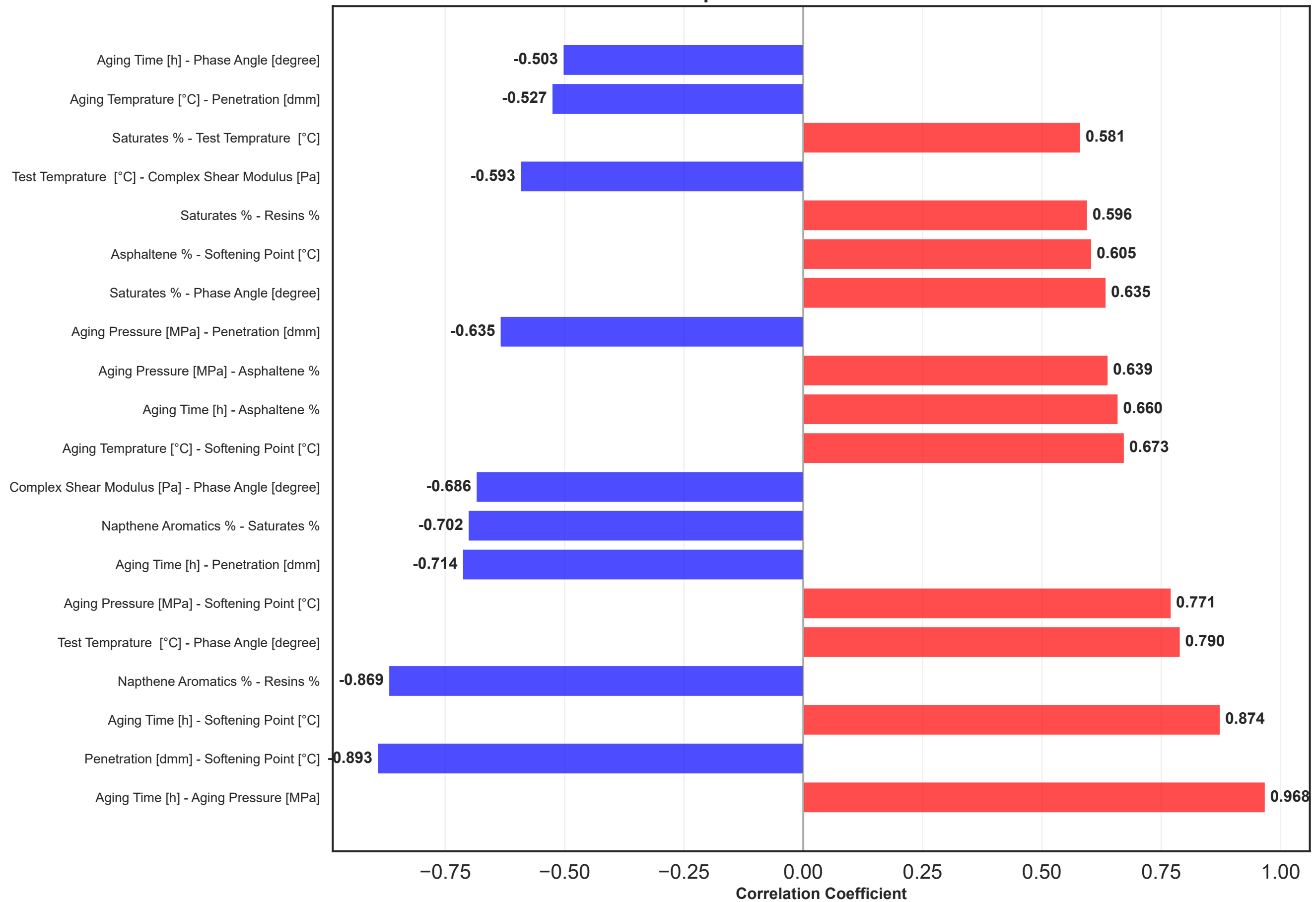
Top 20 Variable Correlations
