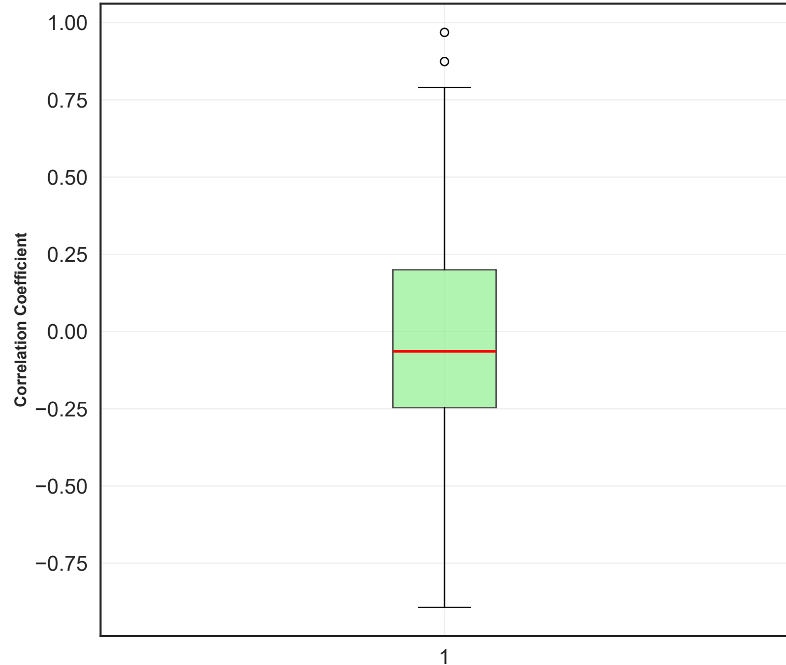
Box Plot of Correlations
