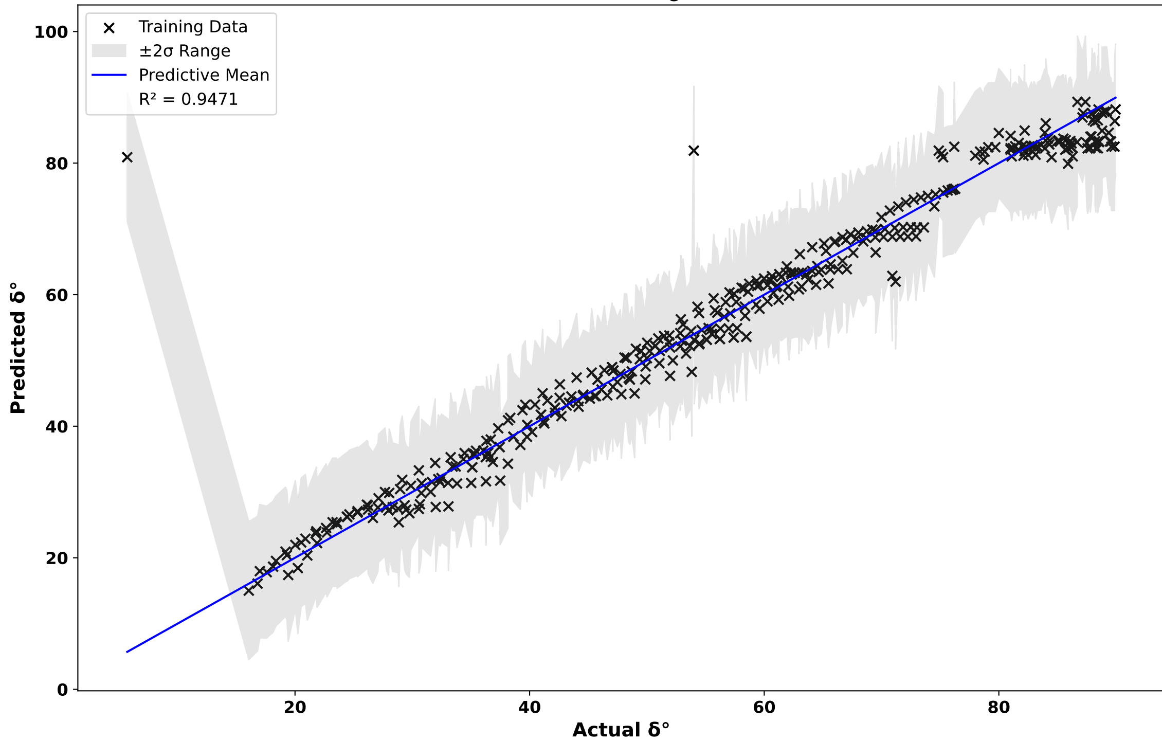
Gaussian Process Regression " \delta "
