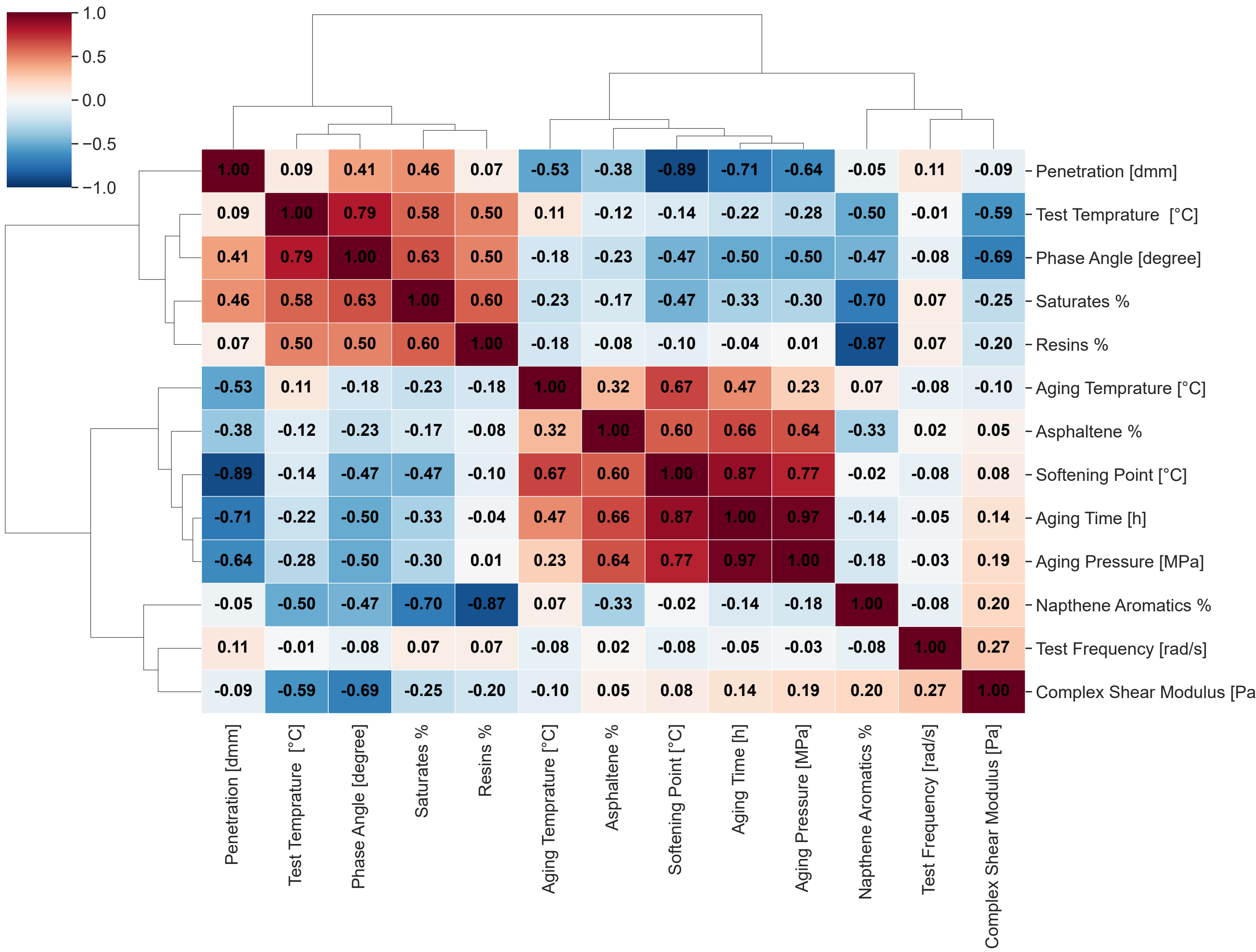
Hierarchically Clustered Correlation Heatmap
