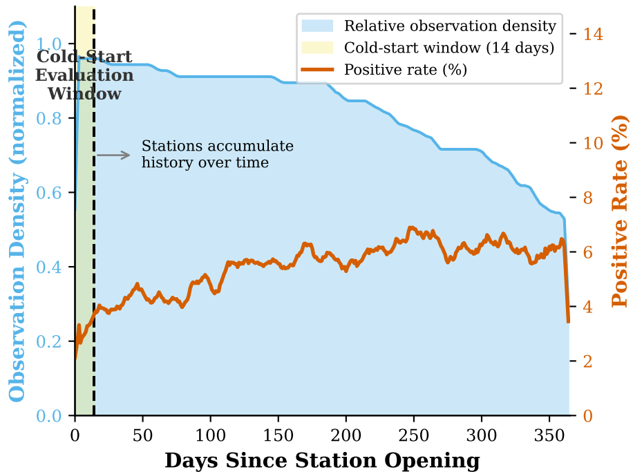
(a) Extreme Zero-Inflation in EV Charging Data (b) Station Lifecycle and Cold-Start Window
