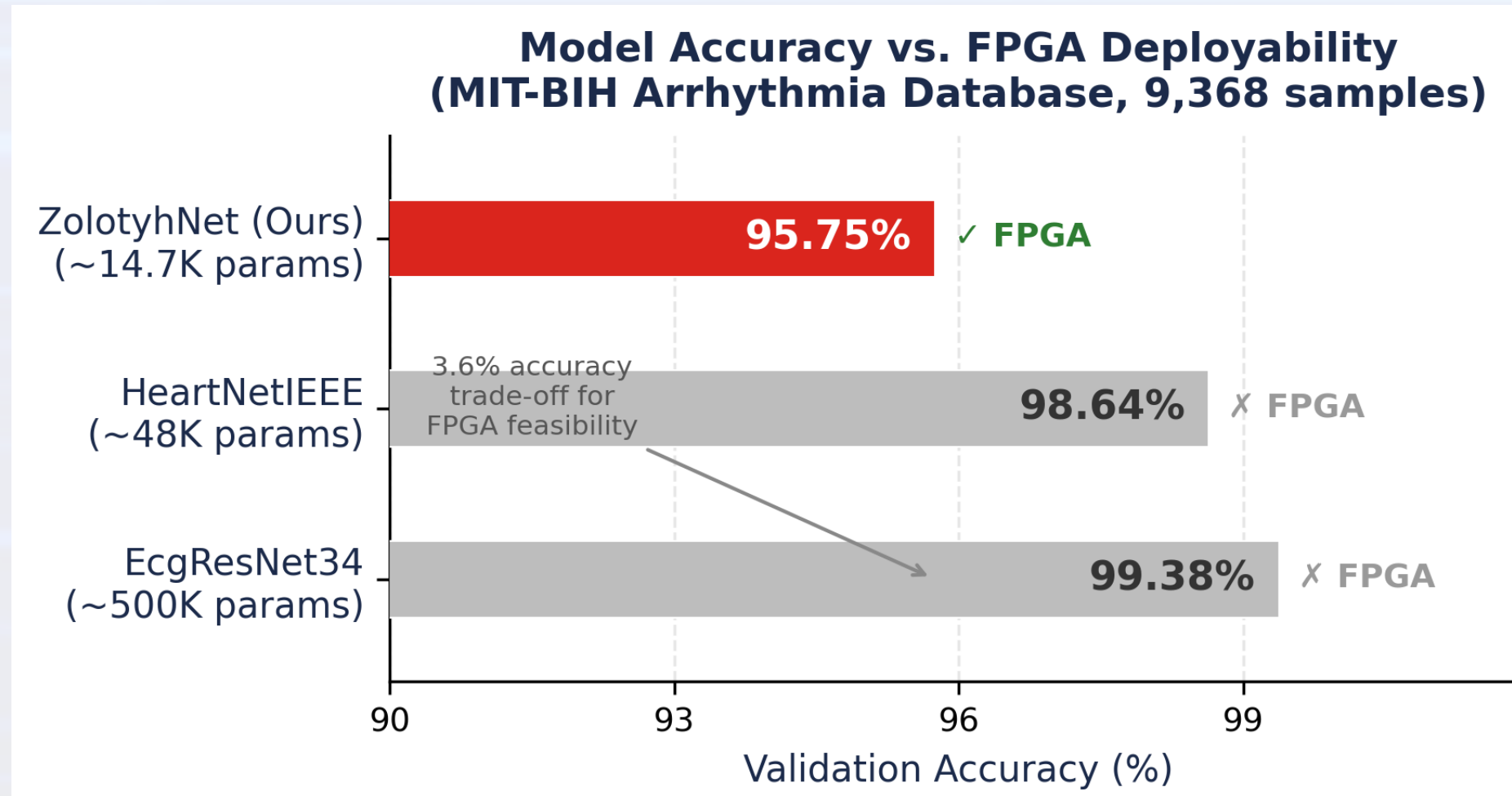
Figure 11: Accuracy comparison.
