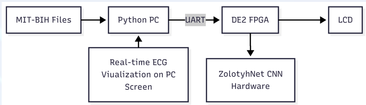
Figure 2: System block diagram.
